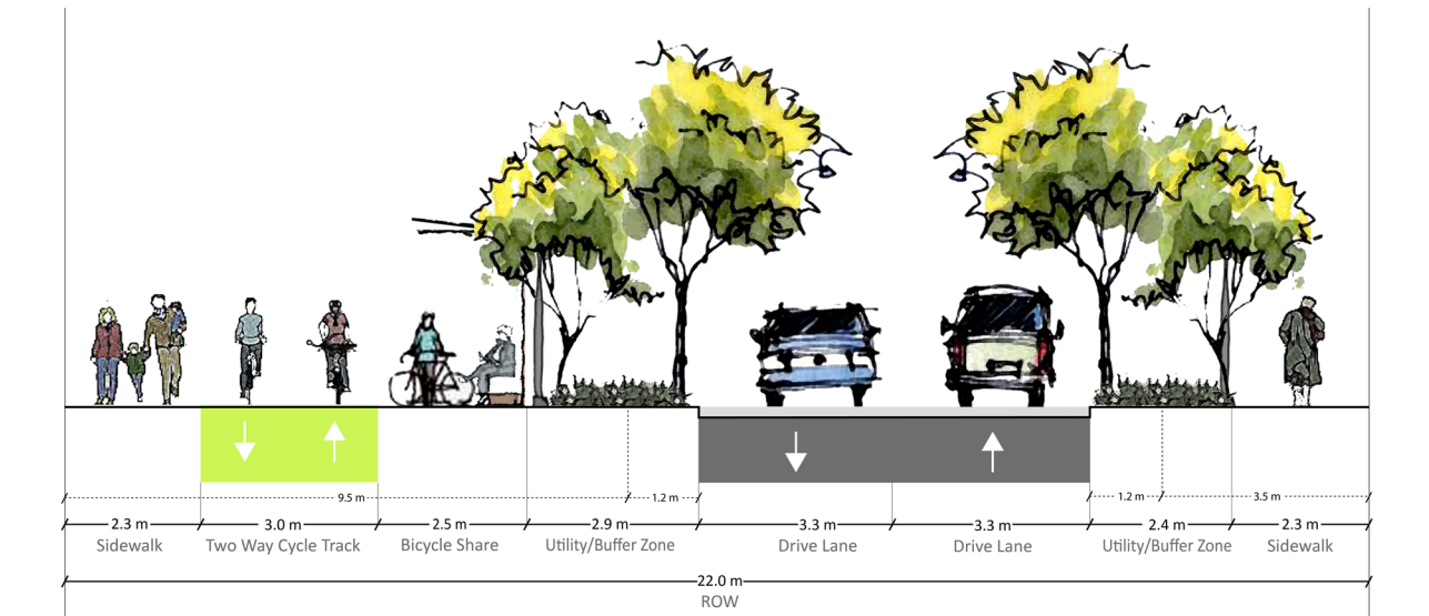
Figure 8.9 Kapyong Minor Collector Street Section with a Bike Share Station
