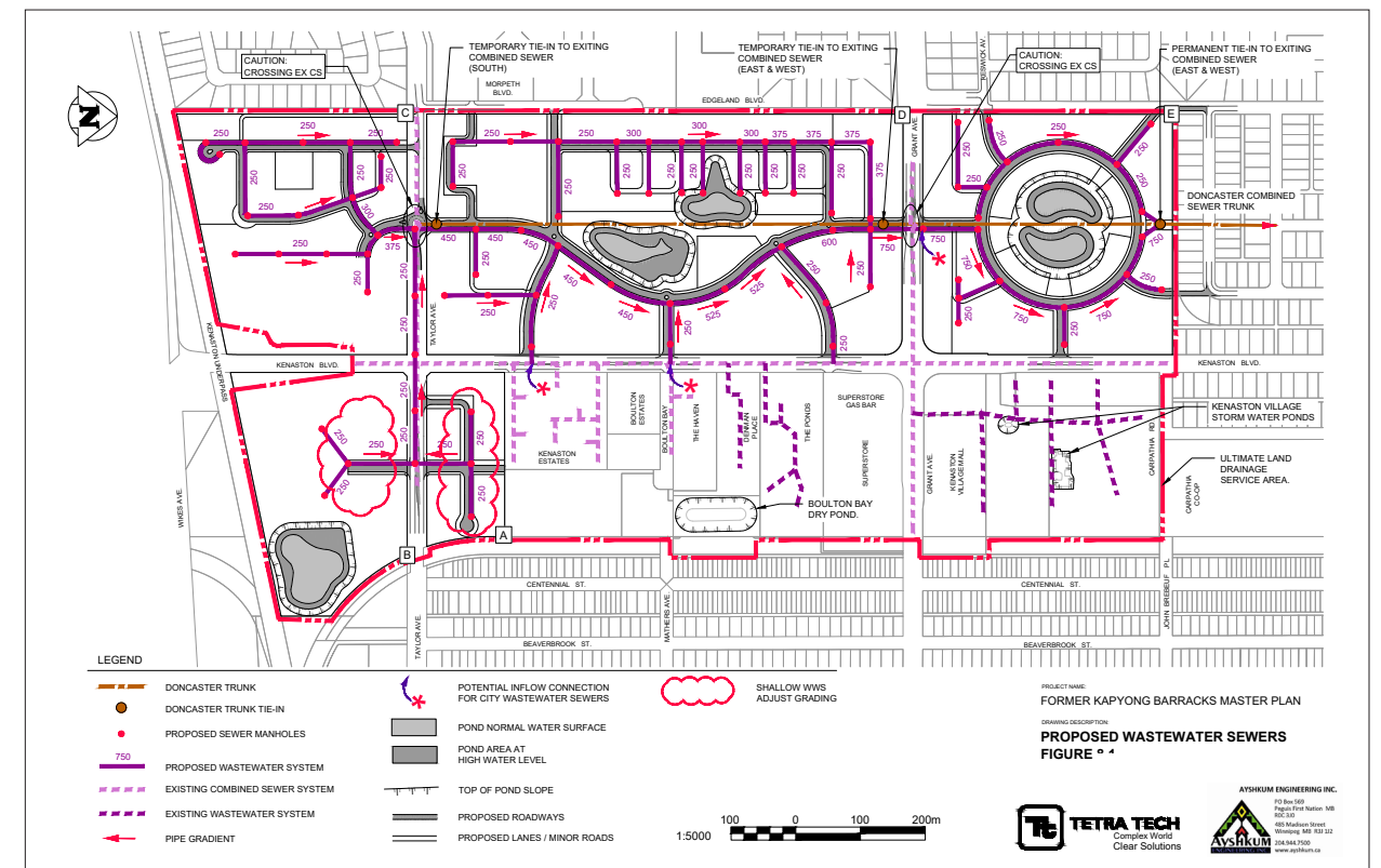
Figure 8.13 Proposed Wastewater Collection
