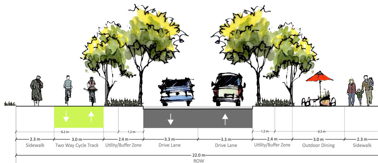
Figure 8.7 Kapyong Minor Collector Street Type B Section with Outdoor Seating
