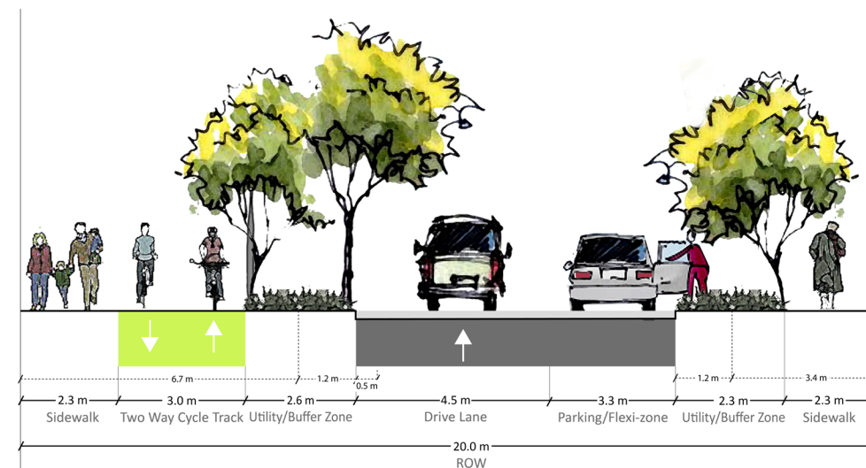
Figure 8.10 Kapyong Minor Collector Type C Street Section with Parking
