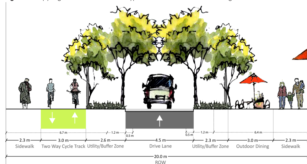
Figure 8.11 Kapyong Minor Collector Street Type C section with Outdoor Seating
