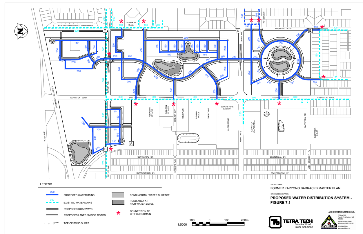
Figure 8.12 Proposed Water Distribution
