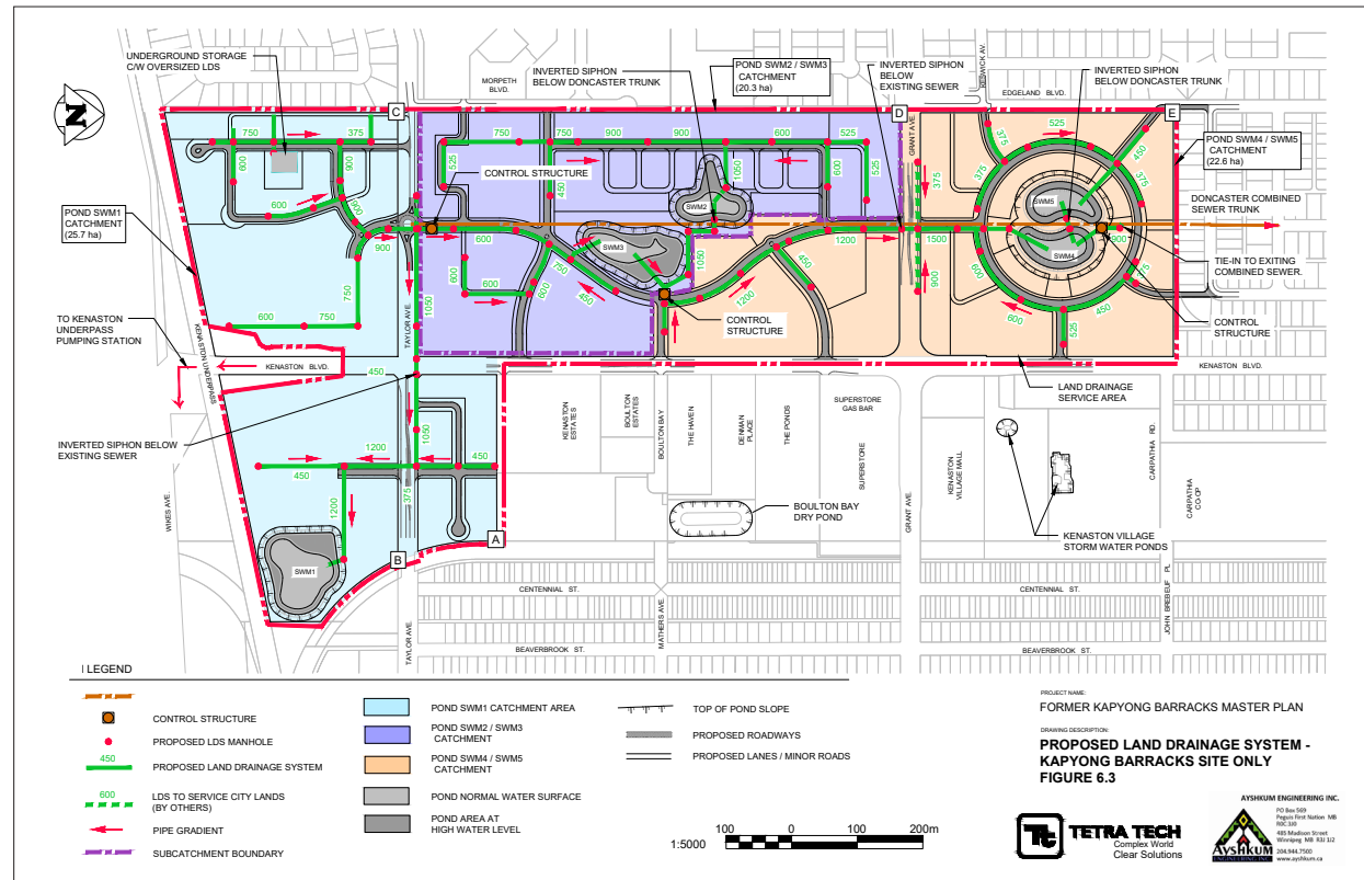
Figure 8.14 Proposed Stormwater Management
