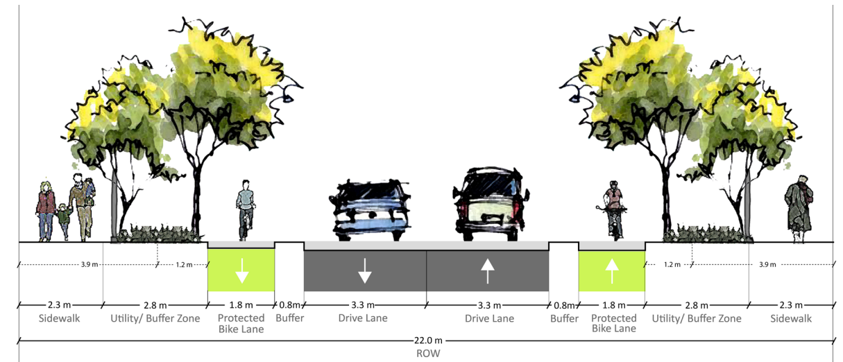
Figure 8.5 Kapyong Minor Collector Type A Street Section
